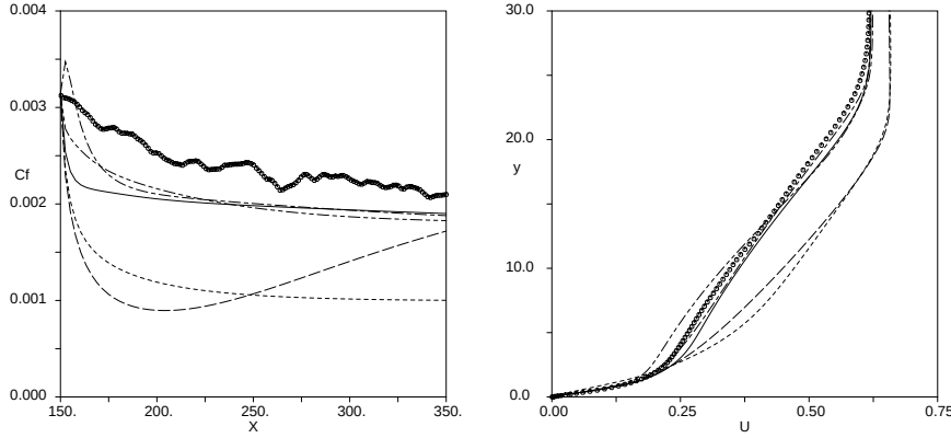
FIGURE 20. (left) The wall skin friction and (right) the velocity profile for an adverse pressure gradient boundary layer ( U_\infty \sim x^{-0.25} ). Computations with standard Wilcox[46] K-\omega (---), Chien K-\varepsilon (---), EARS based on K-\omega and y^+ (.....) or y^* (—) and the Hanjalić[11] RST model (----). Comparisons with DNS data ( \bullet ), Skote (private communication).
