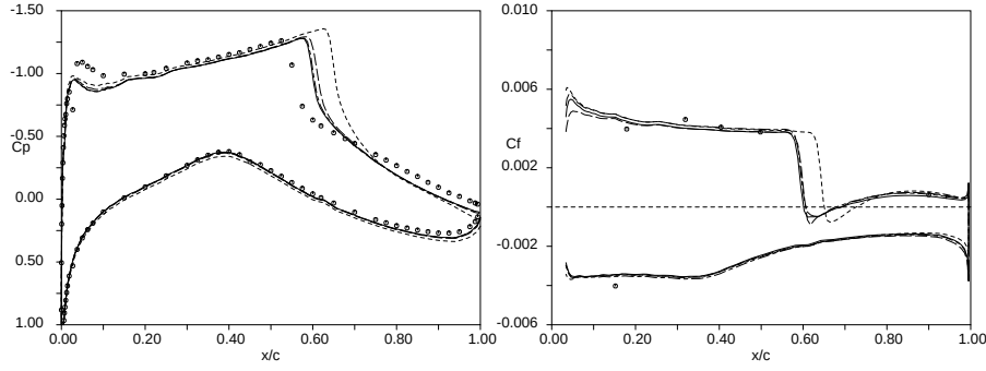
FIGURE 21. Wall pressure and skin friction coefficients for the RAE2822 wing profile ( M = 0.754 , \alpha = 2.57^\circ and Re = 6.2 \cdot 10^6 ). Predictions using Wilcox[48] K-\omega (-----) and the current EARSM based on K-\omega with damping function based on y^+ (---), y^* (—) or without any damping functions (---), compared to experimental data (*) (Cook et al. [2]). The geometry is the measured one including a camber correction.
