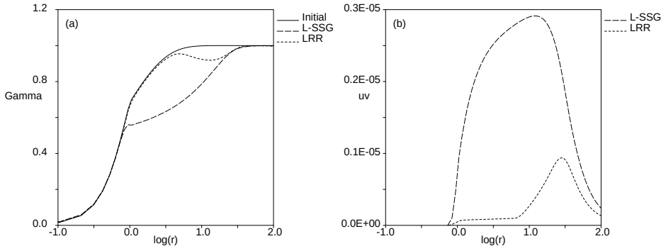
FIGURE 5. The computed vortex circulation (a) and shear stress (b) profiles at t = 55s using different RST models. The flow is initiated using the Proctor profile.
