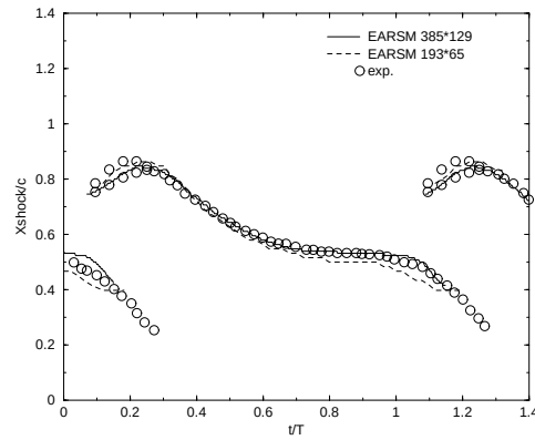
FIGURE 12. Computed shock position using EARSIM on different grids.
