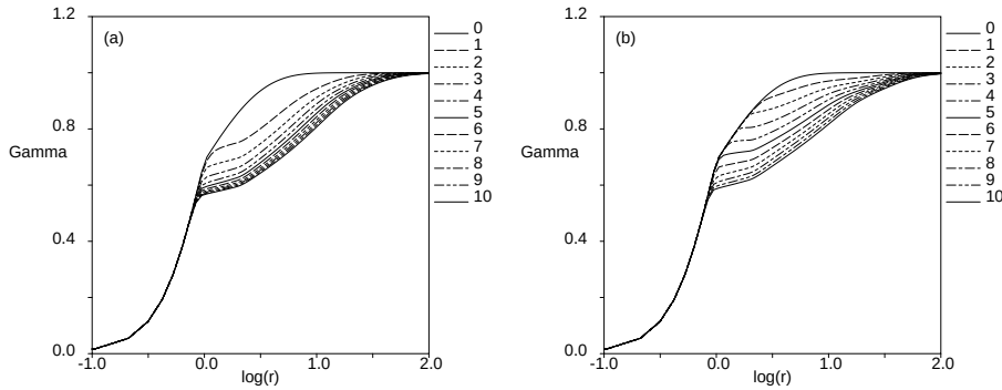
FIGURE 4. The evolution of the computed circulation subjected to different initial turbulent levels using EARSIM based on SSG. (a): High levels where K = 10^{-4} and \varepsilon = 10^{-6} . (b): Nominal levels where K = 10^{-5} and \varepsilon = 10^{-8} . The spacing between each line is 5s.
