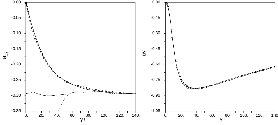
FIGURE 10. a_{12} anisotropy (left) and \overline{uv} stress (right) in channel flow. Comparison of the current EARSM with near-wall correction (—) with DNS data ( \bullet ) by Kim[16]. The computed a_{12} anisotropy using the current EARSM without near wall correction (---) and the eddy-viscosity model (.....) is also shown. The predicted anisotropy was evaluated by use of the DNS data for the \mathbf{S} and \mathbf{\Omega} fields.
