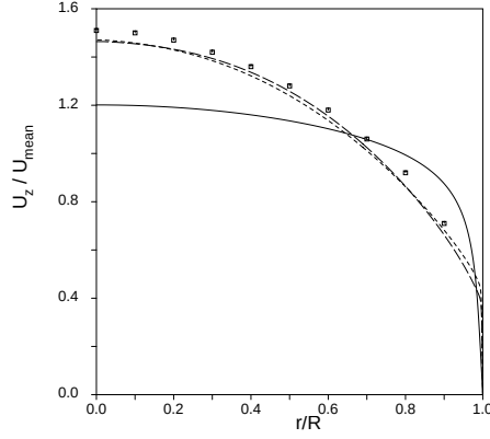
FIGURE 6. Axial velocity in rotating pipe flow for rotation ratio Z = 1 . Computations with Chien K-\varepsilon model (—) and the current EARSMS based on Chien K-\varepsilon , EARSMS_0 (---) and EARSMS_1 (— · — ·), compared to experiment by Imao et al. [14] (■).
