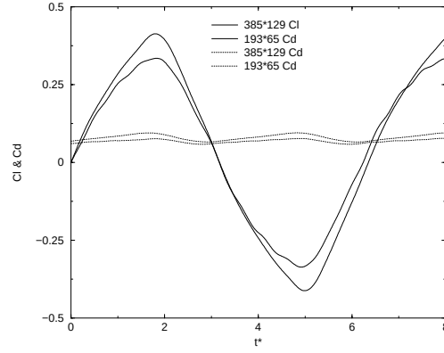
FIGURE 11. Computed lift and drag coefficients using EARSIM on different grids.
