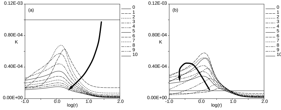
FIGURE 3. The evolution of the computed turbulent kinetic energy subjected to different initial turbulent levels using EARSIM based on SSG. (a): High levels where K = 10^{-4} and \varepsilon = 10^{-6} . (b): Nominal levels where K = 10^{-5} and \varepsilon = 10^{-8} . The spacing between each line is 5s.
