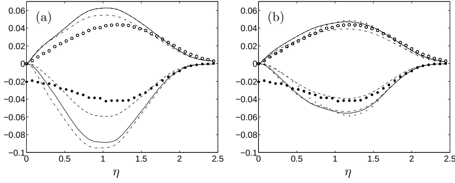
FIGURE 8. Model predictions of the scalar flux components, in the cylinder wake, using the parameter combinations given in Table 1. (a): —, (a); - - -, (b); - · - ·, (e). (b): —, (a r ); - - -, (b r ); - · - ·, (e r ); ···, (a WWJ ). *, \overline{u\theta} ; ○, \overline{v\theta} .
