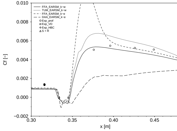
FIGURE 9: Newly developed EARSM using different two-equation model basis. Impinging shock at Mach 5, \beta = 10^\circ , Experiment by Krogmann & Schüle (1996).
