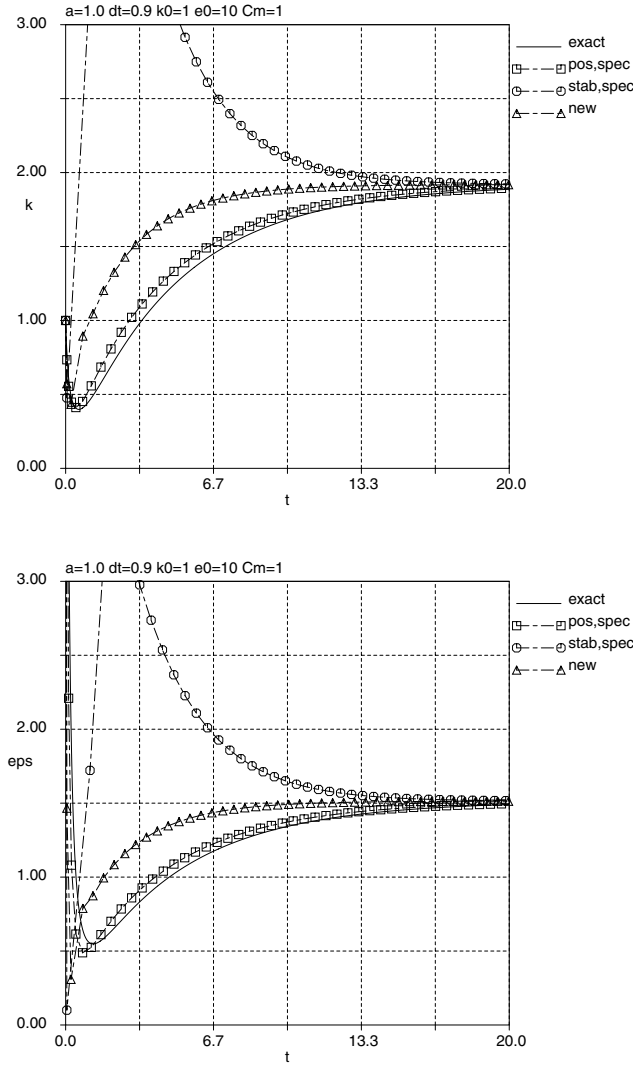
FIGURE 4: Model example with k_0 = 1 , \epsilon_0 = 10 , \alpha = 1 . Time evolution of k (top) and \epsilon (bottom). — exact solution, \square positive time step, \circ stable time step with ‘ad hoc’ resetting, \Delta new proposed time step.
