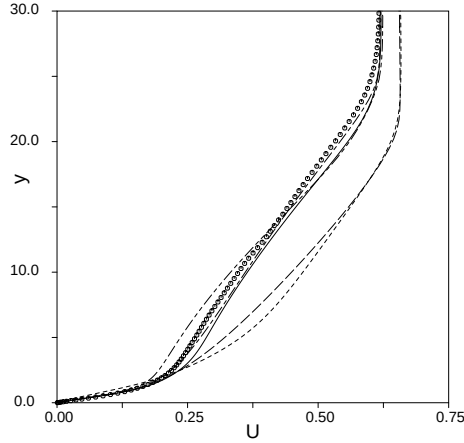
FIGURE 3.5 The velocity profile for an adverse pressure gradient boundary layer ( U_\infty \sim x^{-0.25} ). Computations with standard Wilcox[66] K-\omega (---), Chien[7] K-\varepsilon (-.-), EARSM based on K-\omega and y^+ (.....) or y^* (—) and the Hanjalić[17] RST model (---). Comparisons with DNS data (*), (M. Skote, personal communication)
