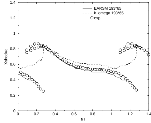
FIGURE 7. Computed shock position using EARSIM and K - \omega compared to experiment[6].
