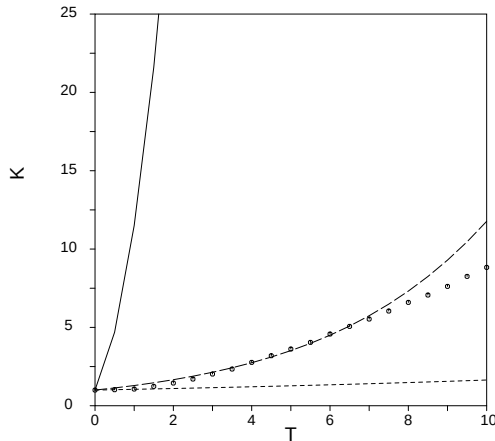
FIGURE 3.2 Time evolution of the turbulent kinetic energy in rapidly sheared homogeneous flow, SK/\varepsilon = 50 . Eddy-viscosity model (—), the Johansson & Wallin[20] self-consistent EARS model (---) and the Gatski & Speziale[12] EARS model (-----) compared with RDT (*).
