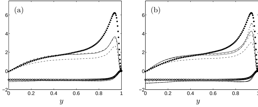
FIGURE 4. Model predictions of the scalar flux components, in the channel flow, using the parameter combinations given in Table 1. (a): —, (a); - - -, (b); - · -, (e). (b): —, ( a^r ); - - -, ( b^r ); - · -, ( e^r ); ···, ( a^{WWJ} ). *, -u\theta ; ○, v\theta from DNS.
