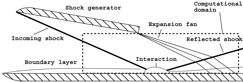
FIGURE 24. Impinging shock at Mach 5. Experimental and computational setup.
