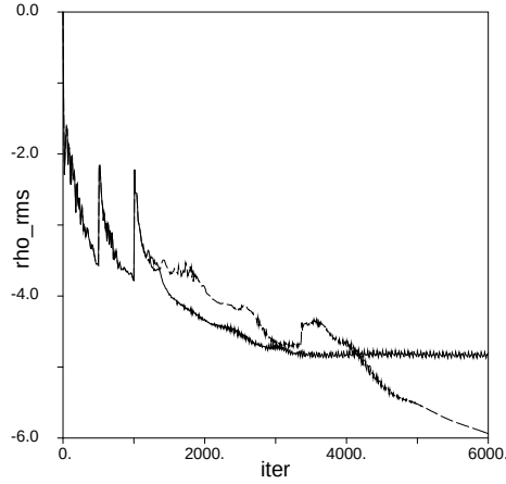
FIGURE 3.7 Convergence history for the RAE2822 wing profile. Wilcox[67] K-\omega (—) compared with the Wallin & Johansson EARSIM based on K-\omega (---). The computational time is increased by 6% by using EARSIM. Three levels of full multigrid is used.
