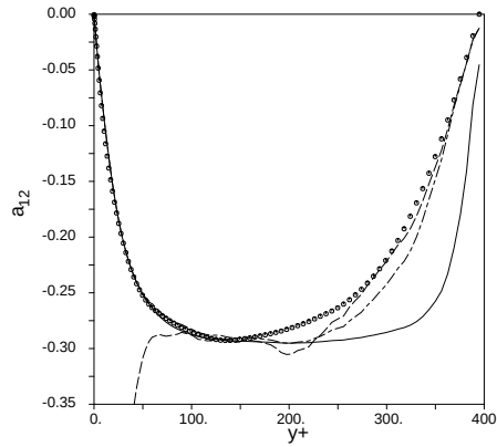
FIGURE 27. The a_{12} anisotropy in channel flow. Comparison of the current EARS model without (—) and with (---) diffusion model with the eddy-viscosity model (— · —) and DNS data (*) by Kim[16].
