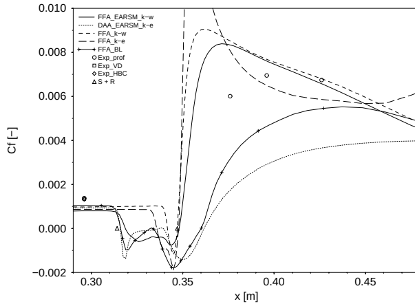
FIGURE 10: Computed skin friction. Impinging shock at Mach 5, \beta = 14^\circ , Experiment by Krogmann & Schüle (1996).
