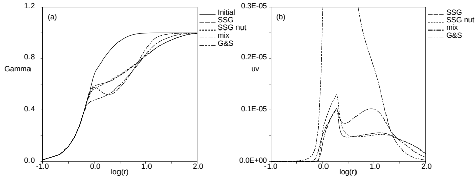
FIGURE 8. The computed vortex circulation (a) and shear stress (b) profiles at t = 55s using different EARSM's based on the linearized SSG model. The flow is initiated using the Proctor profile.
