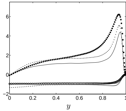
FIGURE 5. Comparison of model ( a^{WWJ} ) and the model of Rogers et al. [22], in the channel flow. —, Rogers et al. ; ···, ( a^{WWJ} ); *, -u\theta from DNS; ○, v\theta from DNS.
