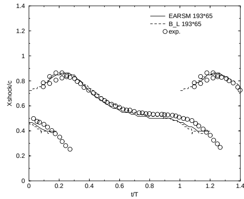
FIGURE 8. Computed shock position using EARSIM and Baldwin-Lomax compared to experiment[6].
