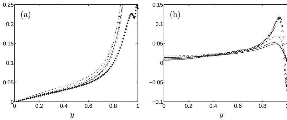
FIGURE 3. Model predictions of \Pi_{\theta_i} - \varepsilon_{\theta_i} in the channel flow, using the parameter combinations given in Table 1. (a): —, (a r ); - - -, (b r ); - · - ·, (e r ); ···, (a WWJ ); *, \Pi_{\theta_1} - \varepsilon_{\theta_1} from DNS. (b): —, (a r ), (b r ); - · - ·, (e r ); ···, (a WWJ ); ○, \Pi_{\theta_2} - \varepsilon_{\theta_2} from DNS.
